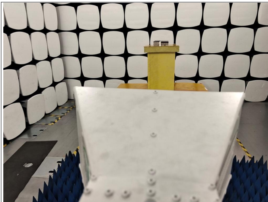
Radiated spurious emissions at frequencies 1 GHz-18GHz
