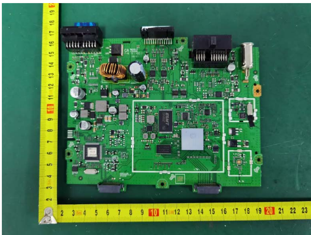
Internal photos M/N: JRV9100
