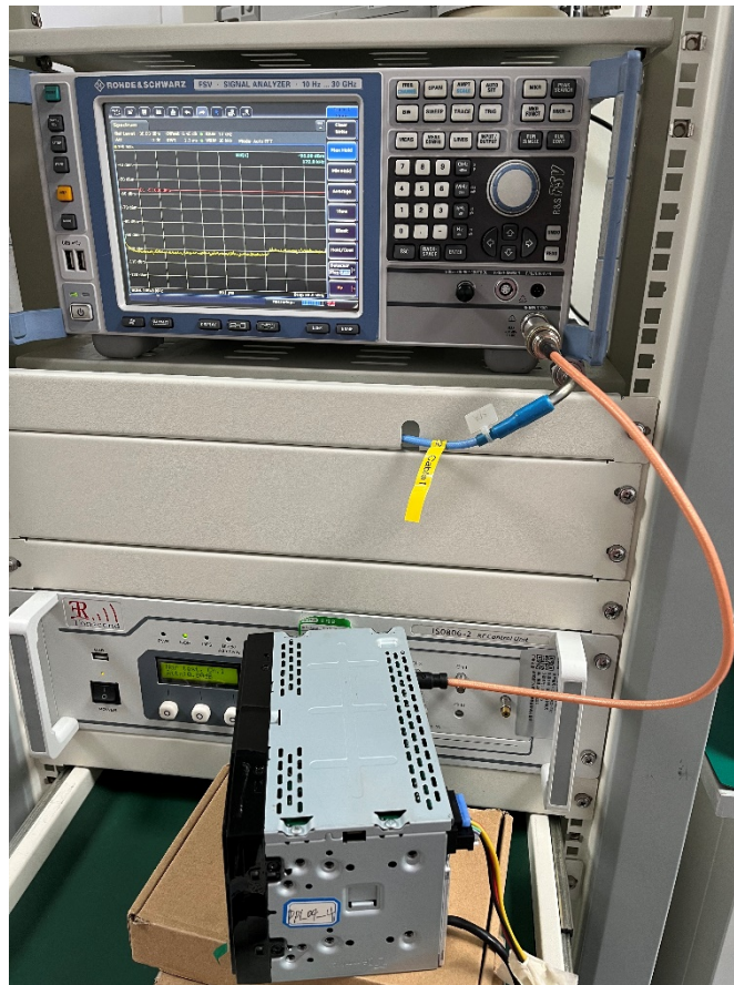
Description: Conducted Test Setup Photo
