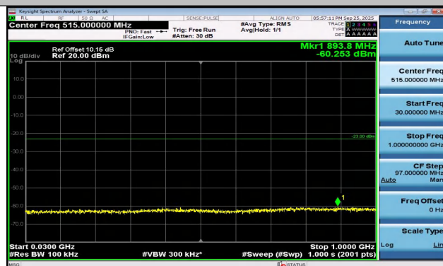
Band4-5MHz-QPSK-20375-25RB#0-30~1000-PASS
