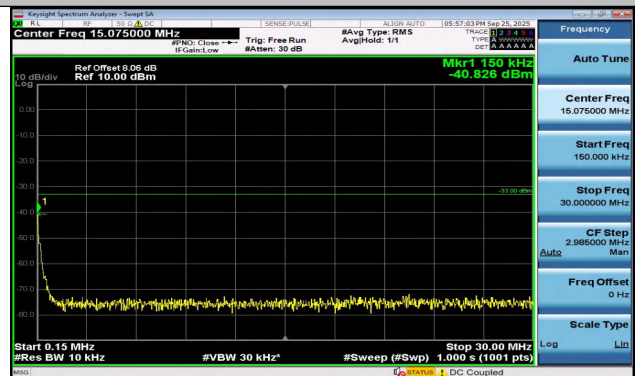
Band4-5MHz-QPSK-20375-25RB#0-0.15~30-PASS
