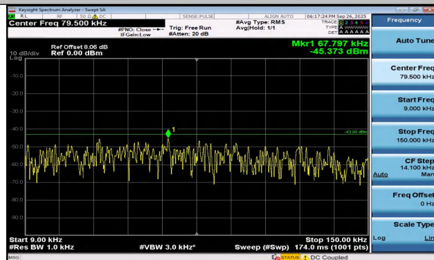
Band4-5MHz-QPSK-20375-25RB#0-0.009~0.15-PASS
