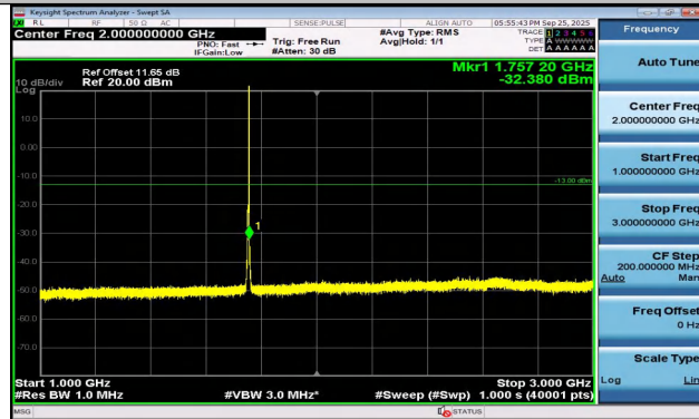
Band4-5MHz-QPSK-20375-1RB#24-1000~3000-PASS
