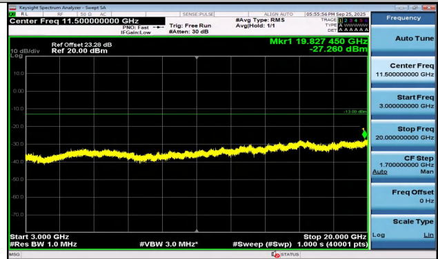
Band4-5MHz-QPSK-20375-1RB#24-3000~20000-PASS
