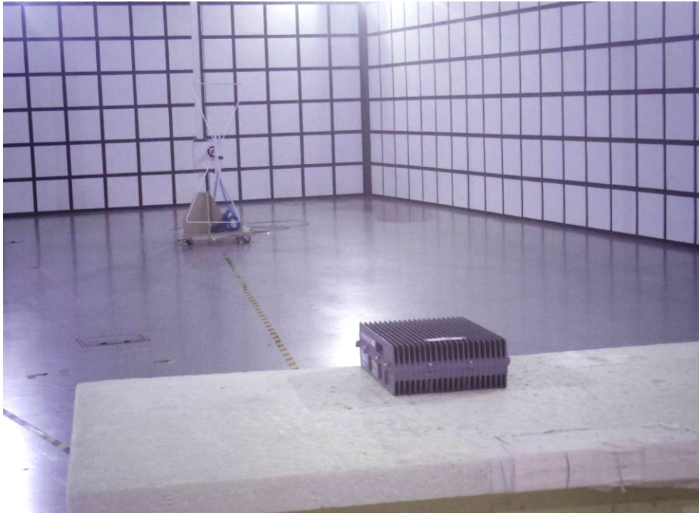
30MHz ~ 1GHz Radiated Emission
