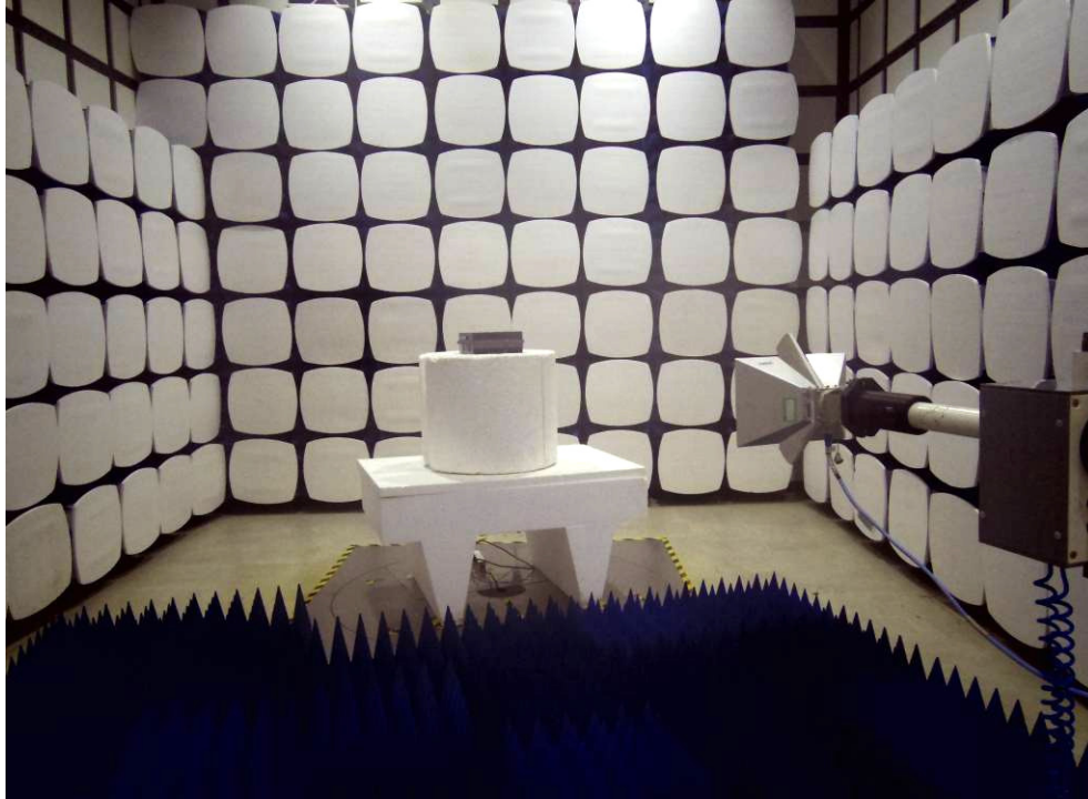
Above 1GHz Radiated Emission
