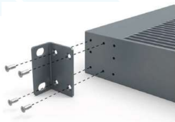
Attaching a 19" Mounting Bracket
