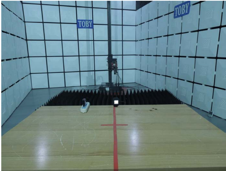
Photo of Setup for Radiated Emission Above 1G
