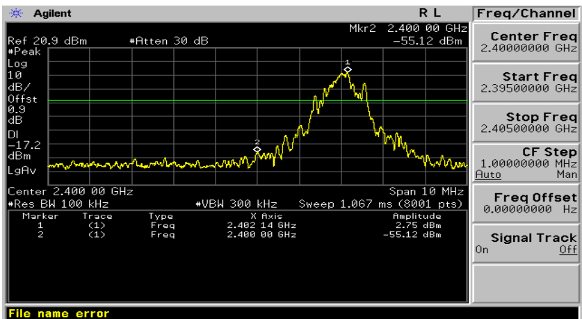
8DPSK/LCH/No Hop
