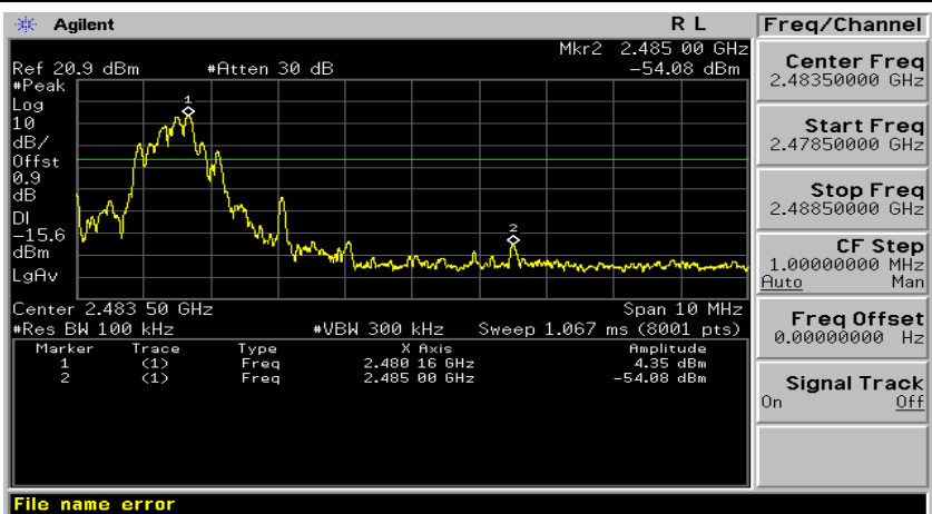
8DPSK/HCH/No Hop
