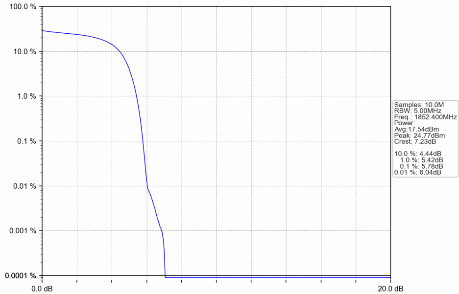
Band2_HSUPA_LCH_1852.4MHz_Subtest 1_NTNV
