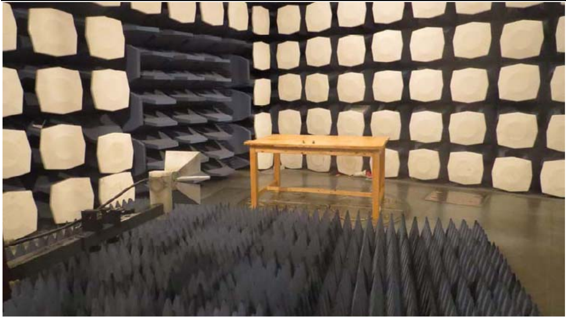
Above 1GHz
