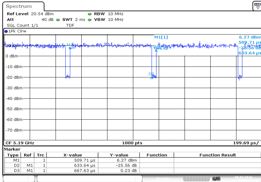
Plot 3: duty cycle of the transmitter – OFDM / n HT40 – mode
