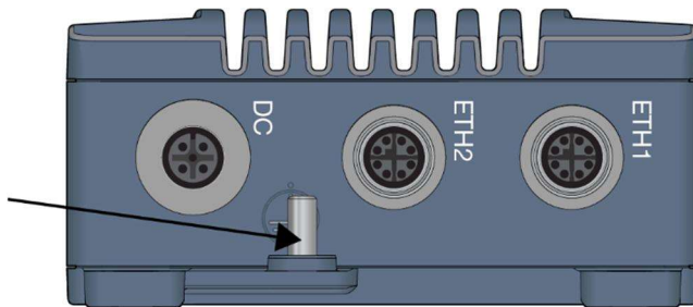
Figure 9 Earth connection
