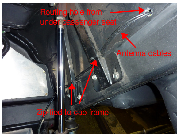
Figure 16: Zip-tie to frame under elevated cab
