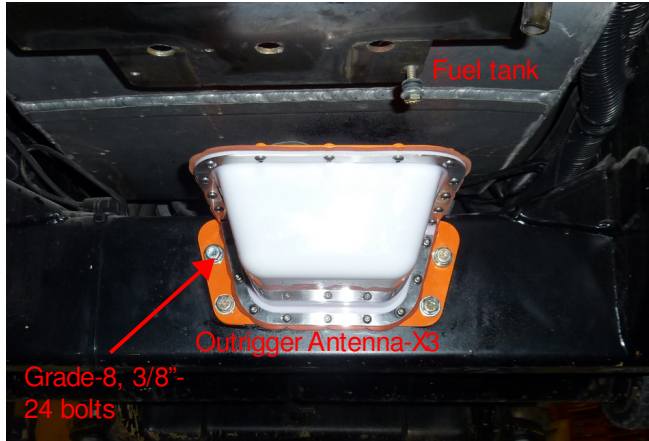
Figure 14: Outrigger Antenna mounted parallel to ground
