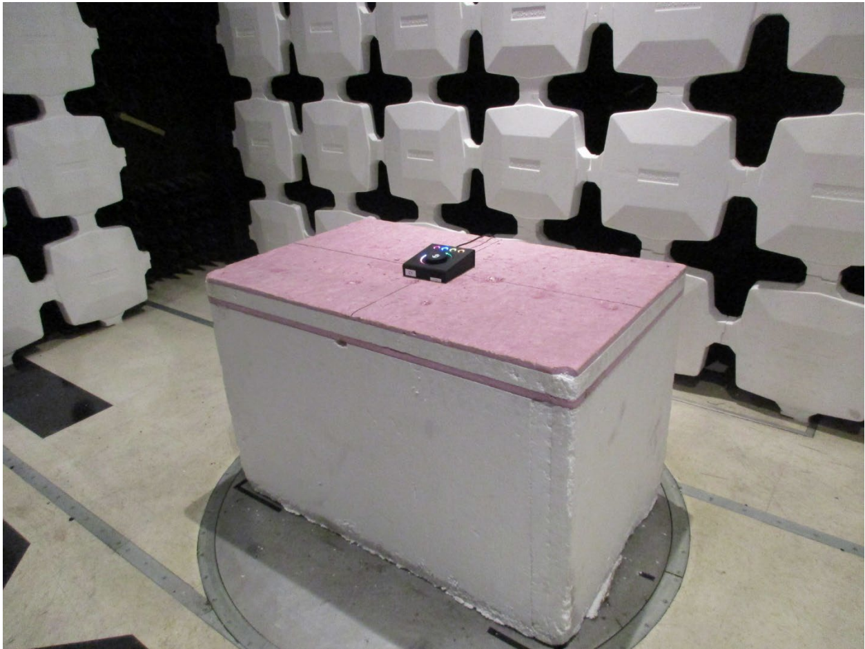
Radiated Testing, Table Setup
