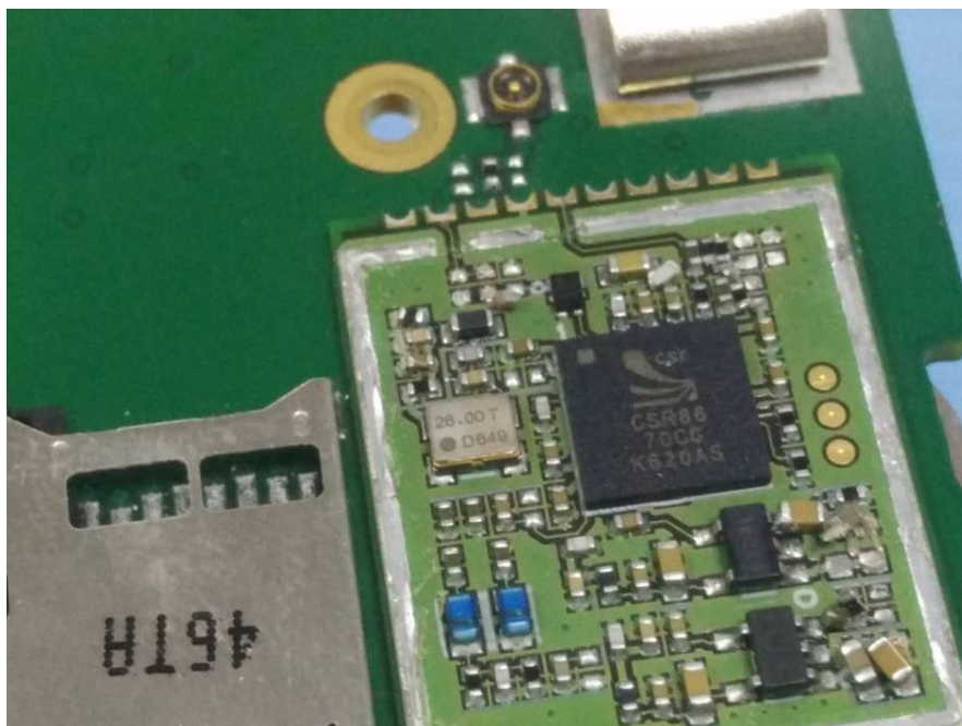
EUT – BT IC View
