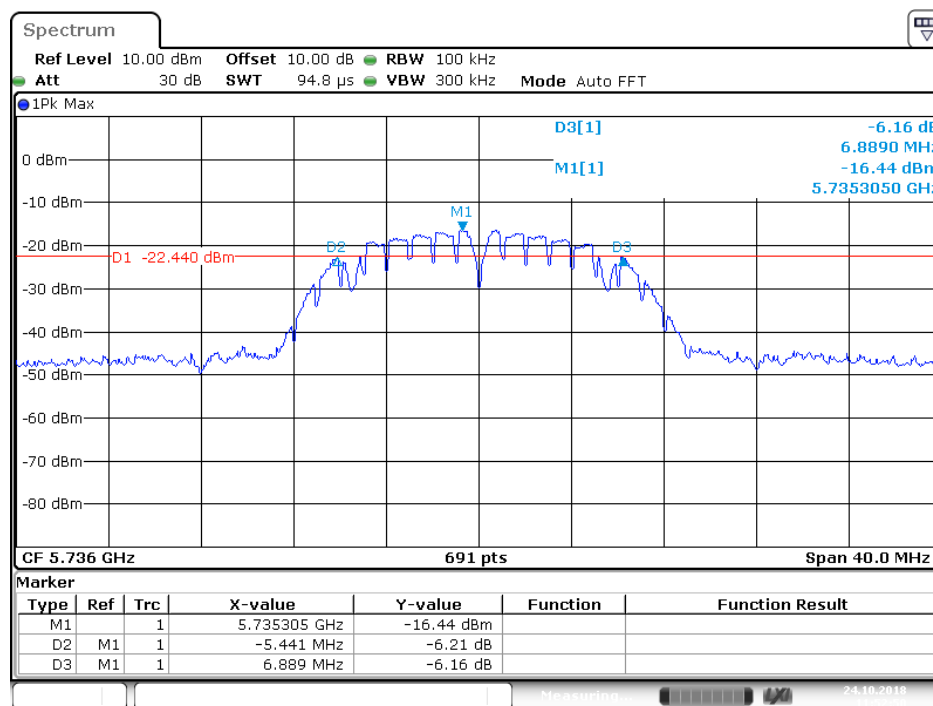
Low channel(Antenna A)
