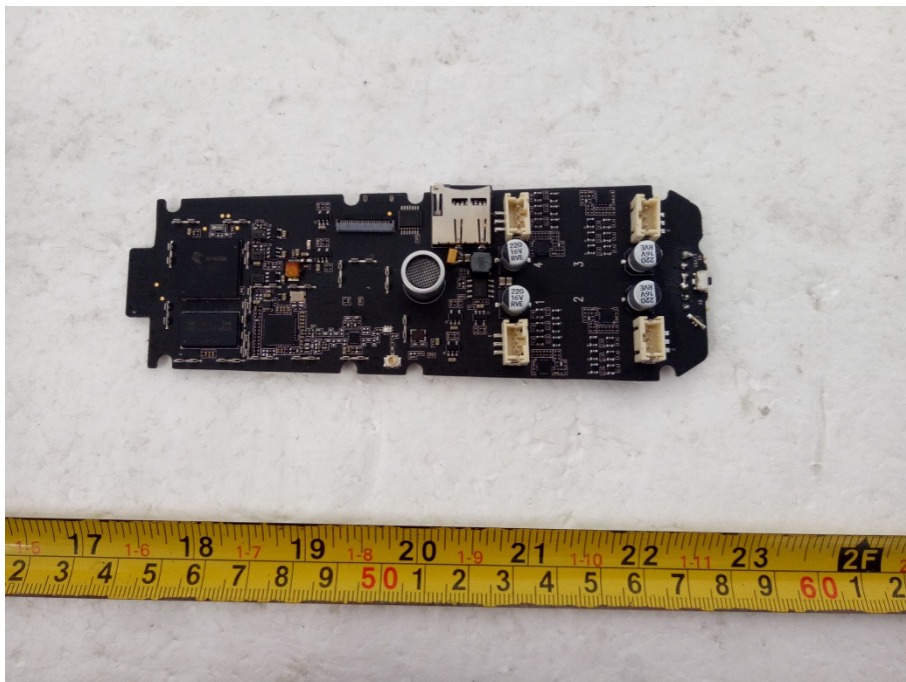
EUT –Main Board-3 Shielding off View
