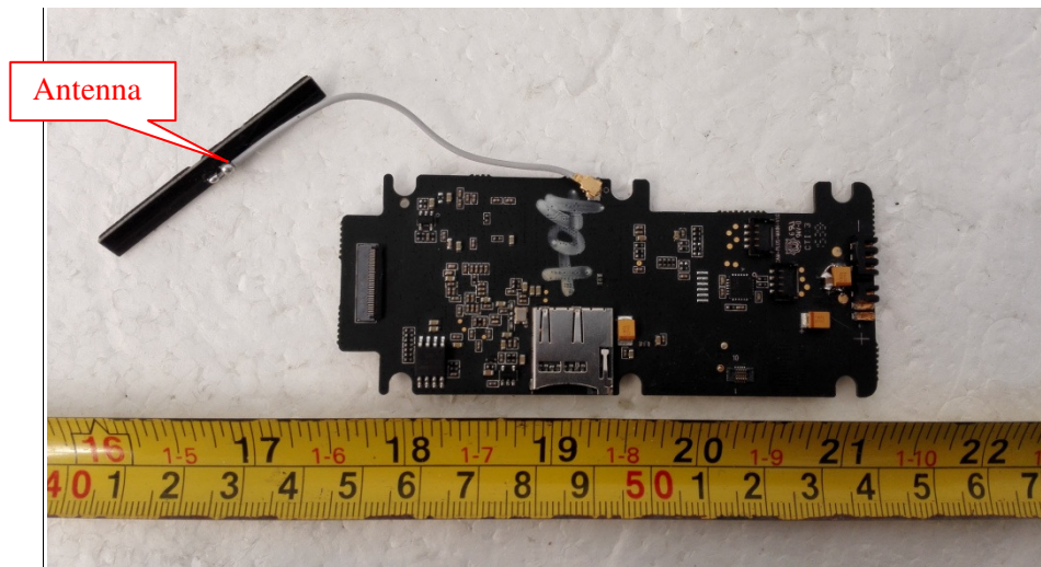
EUT –Main Board-3 Top View
