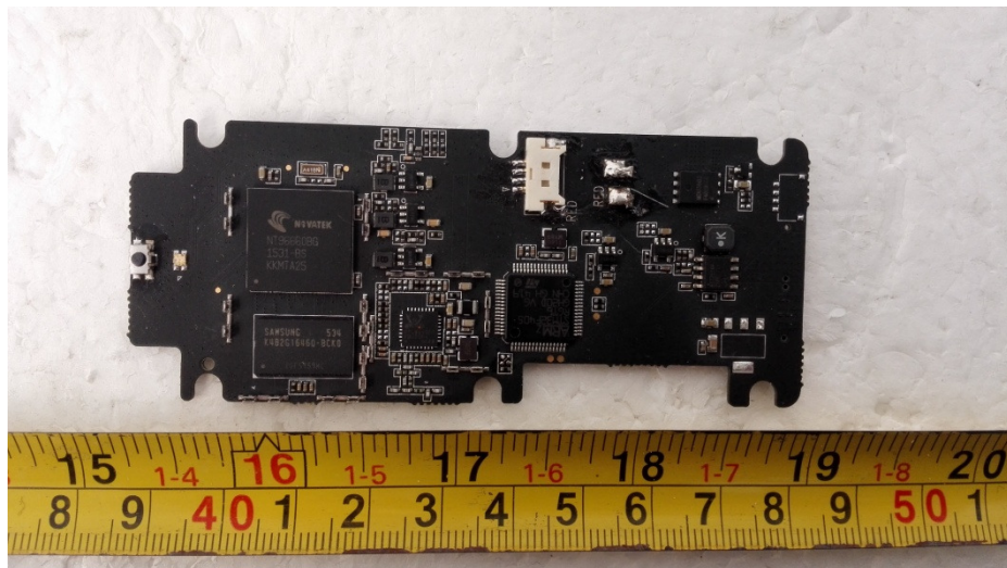
EUT –Main Board-3 Shielding off View
