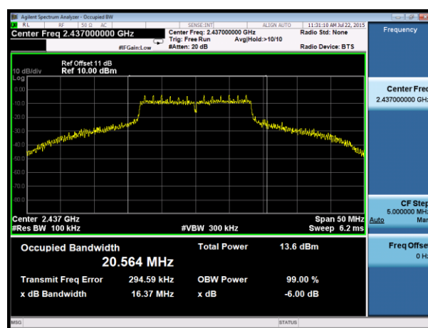
Channel 06 (2437MHz)
