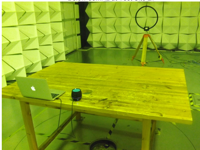
Photograph – Radiation Spurious Emission Test Setup
