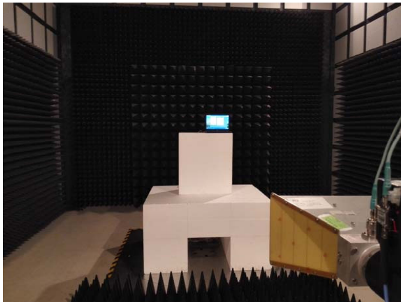
Radiated Spurious Emissions View (Above 1 GHz)
