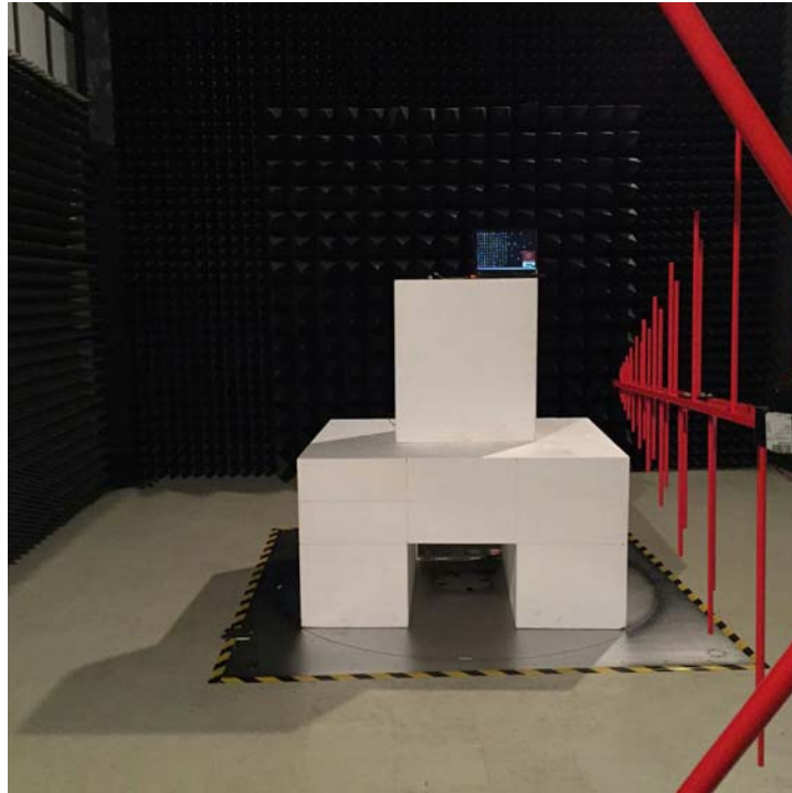
Radiated Spurious Emissions View (Below 1 GHz)
