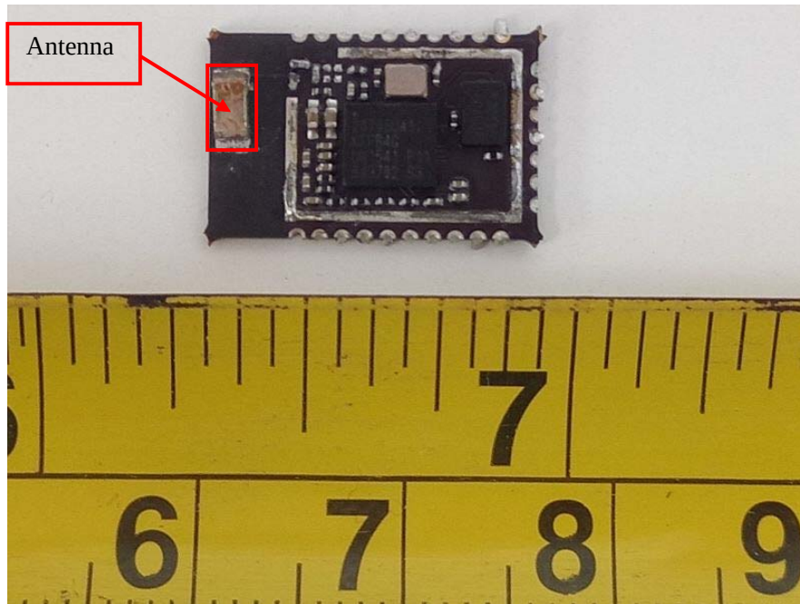
EUT –Shielding Cover off View
