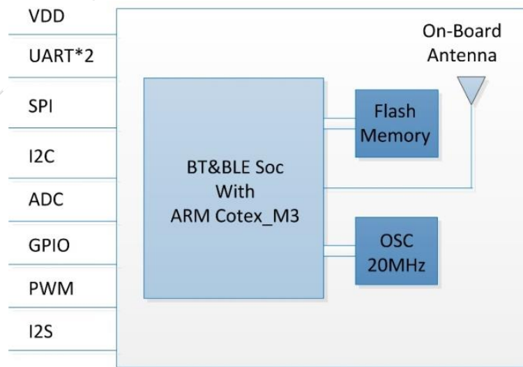
Figure 1 - Block Diagram
