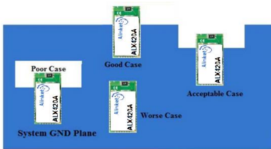
Figure 12 - Antenna Design
