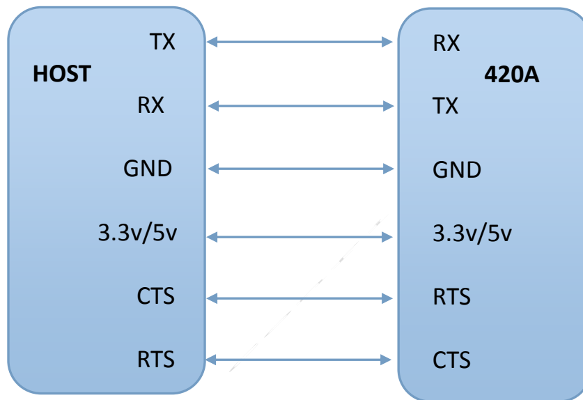
Figure 5 - Detail Connection
