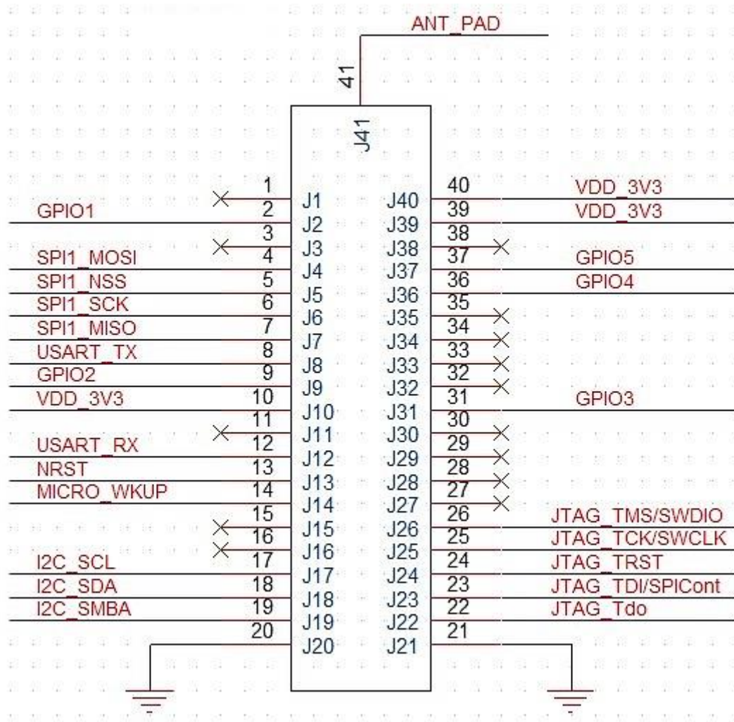
Figure 4 Ball Maps
