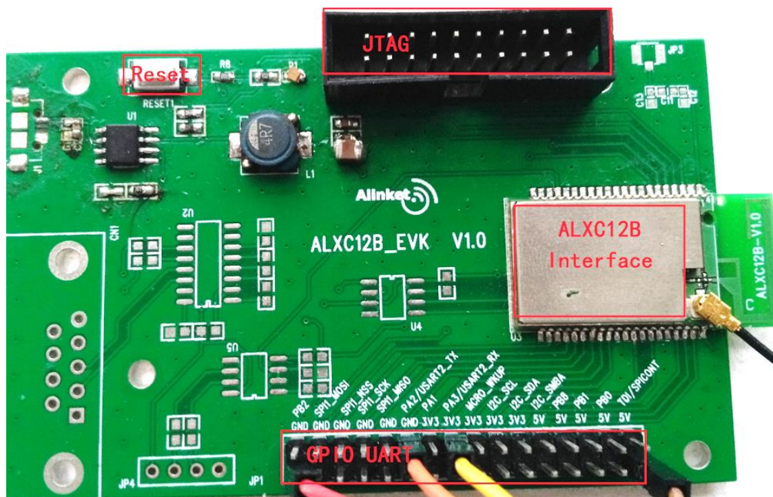
Figure 14 ALXC12B EVK
