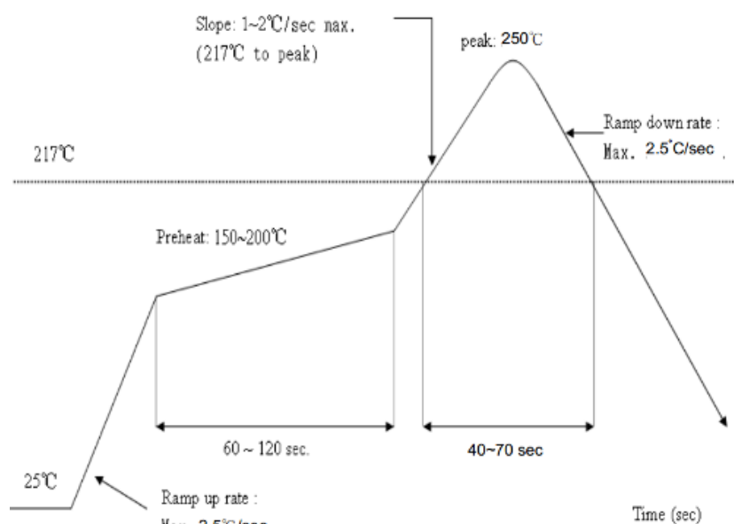
Figure 45 Reflow Profile
