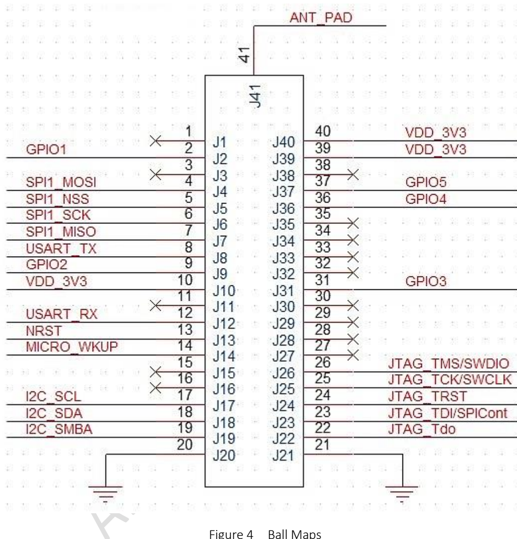
Figure 4 Ball Maps
