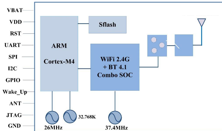
Figure 2 Block Diagram
