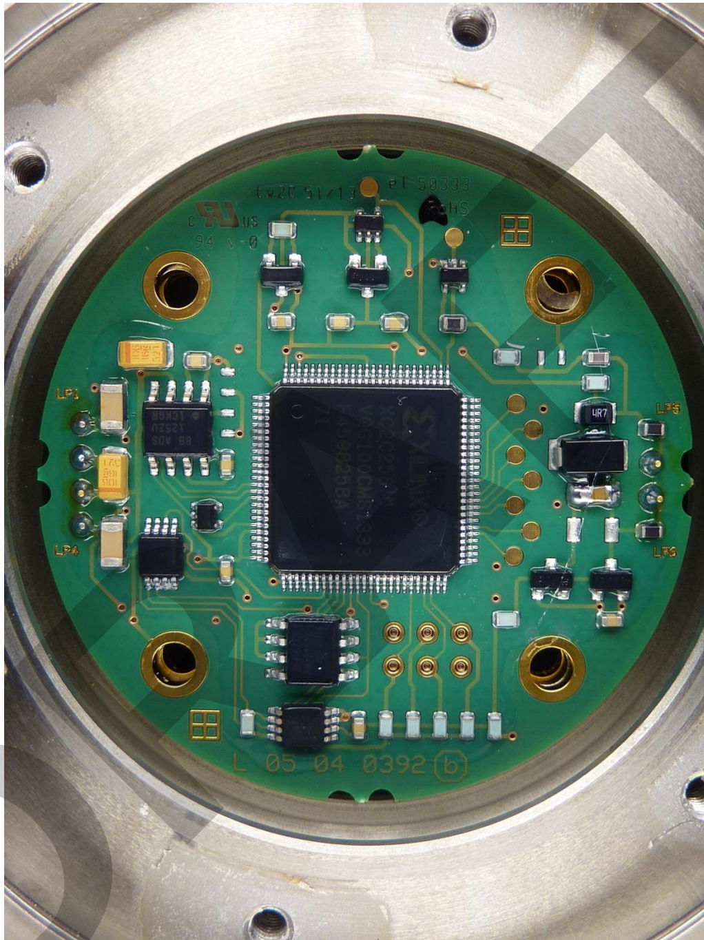
147045_m.JPG: 4550A1K0S10N1WA, PCB, top view
