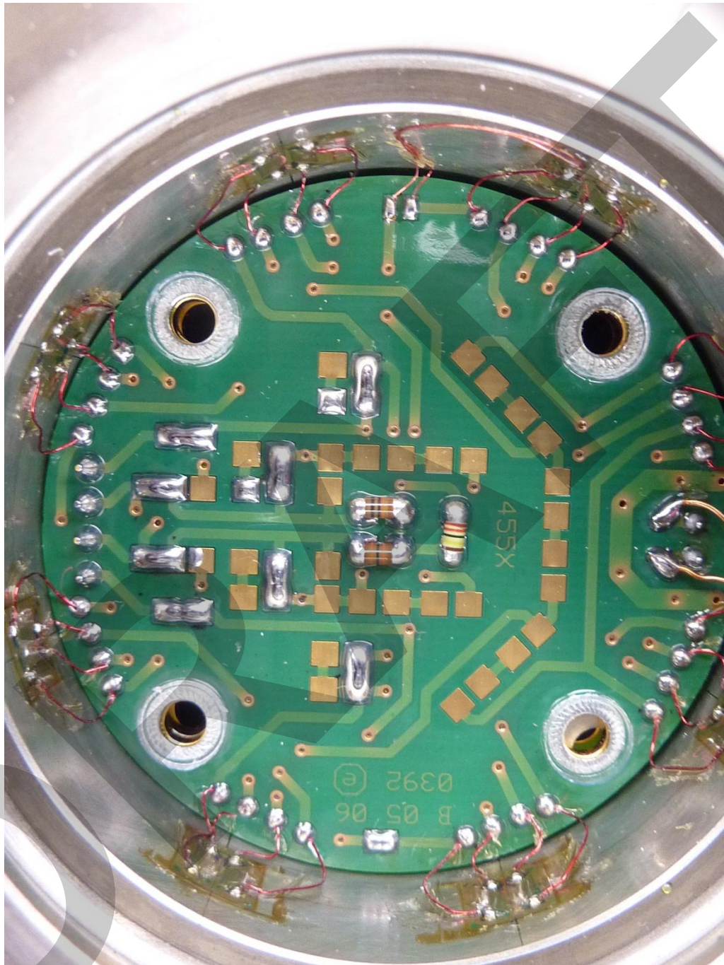
147045_n.JPG: 4550A1K0S10N1WA, PCB, bottom view
