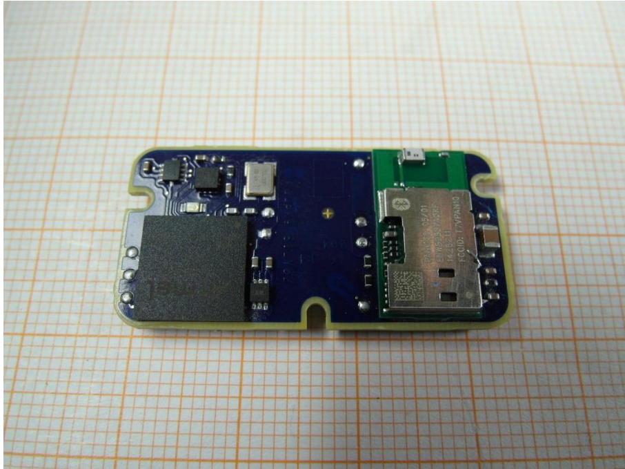
Photo 1: periphery electronic with BT module an ceramic chip antenna
