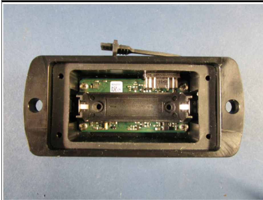
EUT-Disassembly 2
