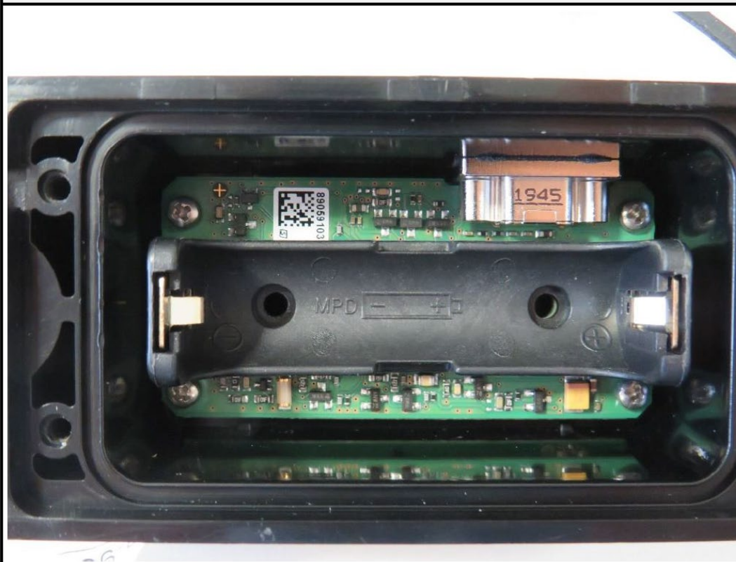
PCB TOP SIDE WITHOUT BATTERY
