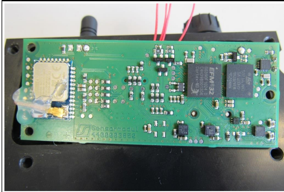
EUT PCB with external Antenna Back
