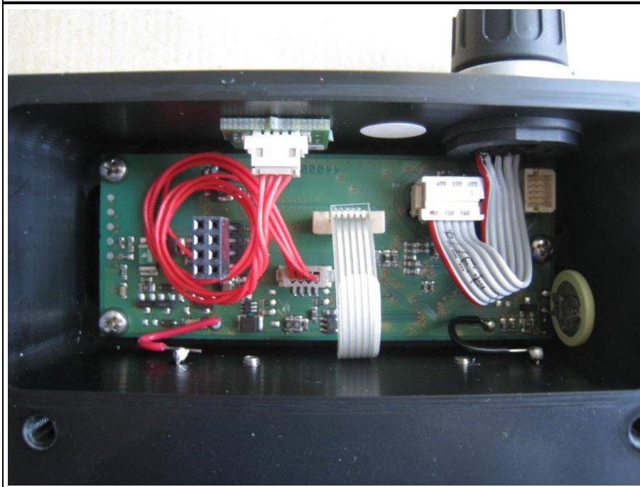
EUT with internal Antenna open
