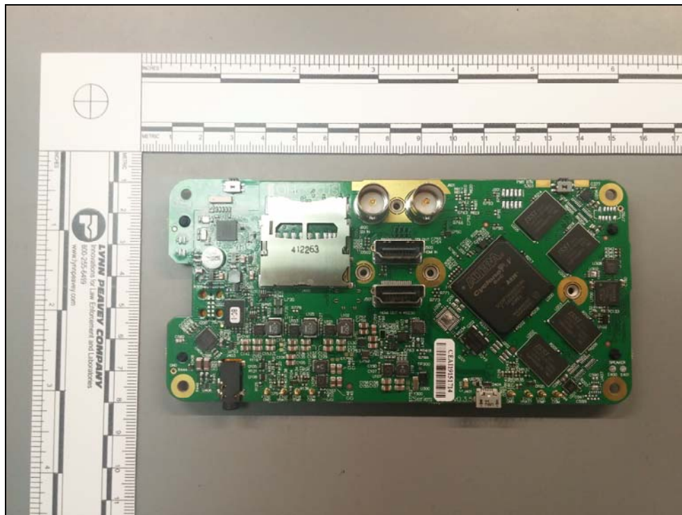
Figure 3: M502 Mainboard Back View
