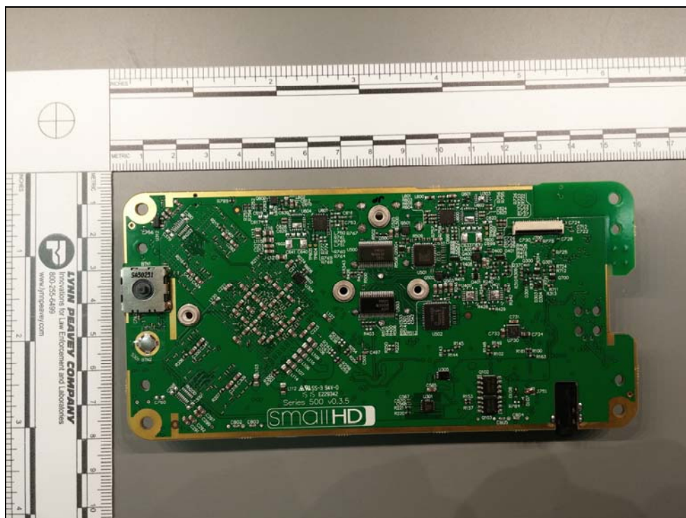
Figure 4: M502 Mainboard Front View
