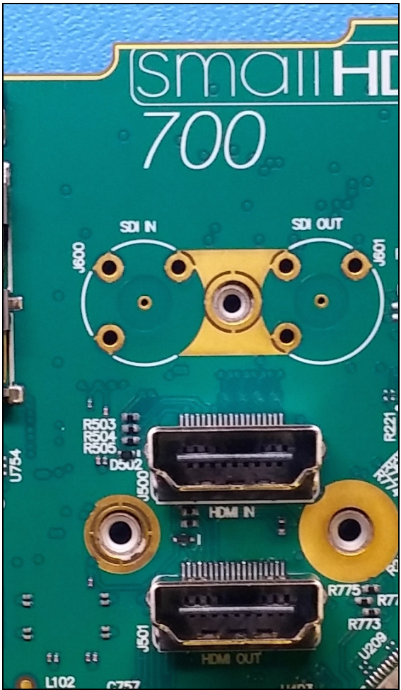
Figure 2: Model 701- Mainboard - Rear Differences (BNC Connectors)
