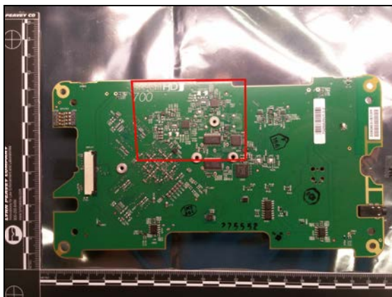
Figure 5: Model 702 - Mainboard - Front With region of differences vs 701
