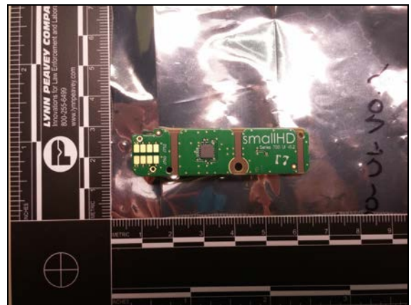
Figure 10: Common UI Board - Rear
