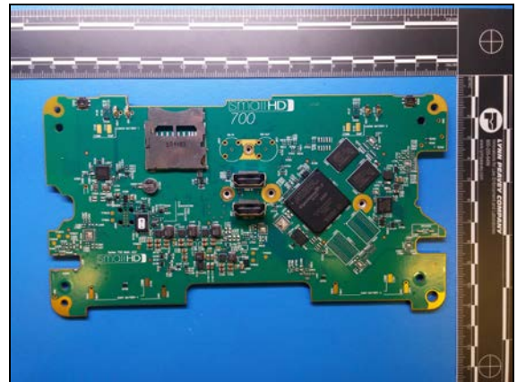
Figure 4: Model 701L- Mainboard - Rear
