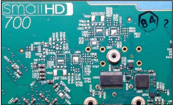
Figure 1: Model 701- Mainboard Front Differences (SDI Circuits)
