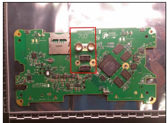
Figure 6: Model 702- Mainboard - Rear With region of differences vs 701
