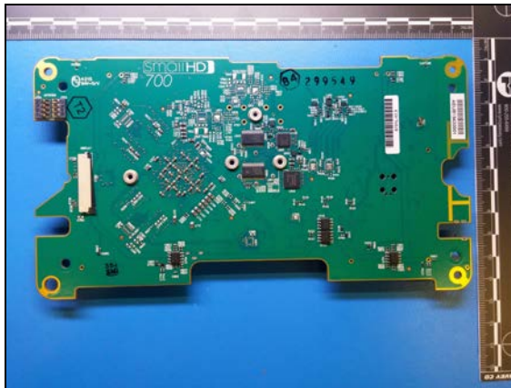
Figure 3: Model 701L- Mainboard - Front
