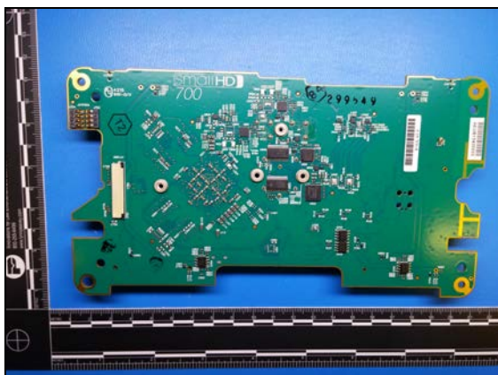
Figure 7: Model 702L- Mainboard - Front
