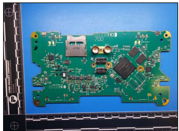
Figure 8: Model 702L- Mainboard - Rear
