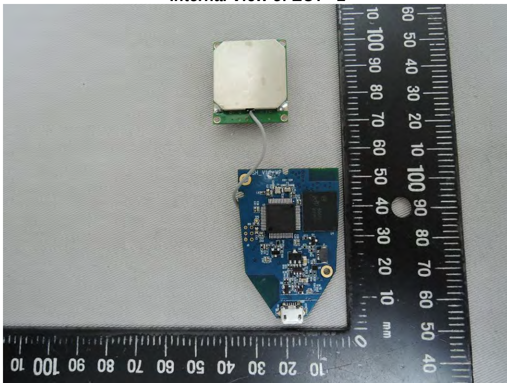
WLAN / GPS Antenna
