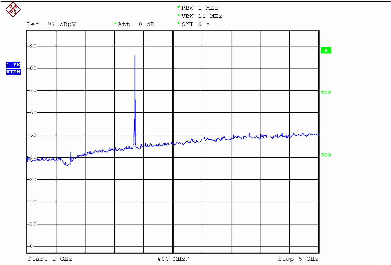
Fig B4 High Channel Radiated Emissions 1GHz -5GHz Horizontal 3metres
