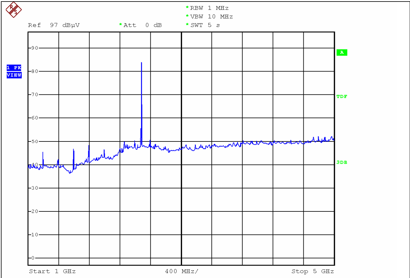
Fig B3 High Channel Radiated Emissions 1GHz -5GHz Vertical 3metres
