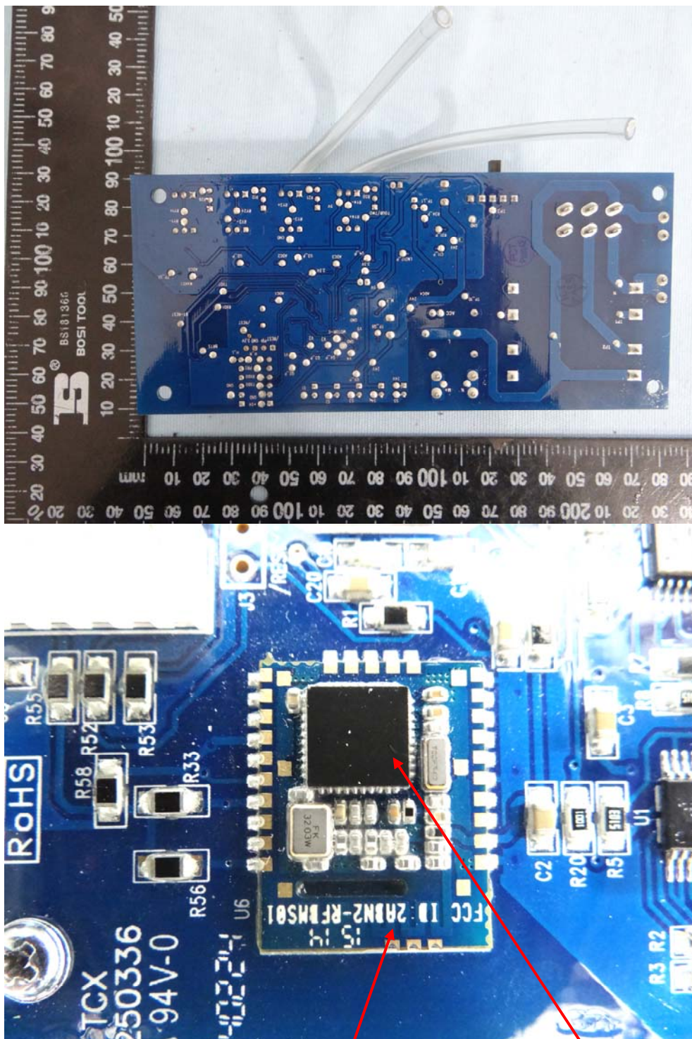
BT Chip
