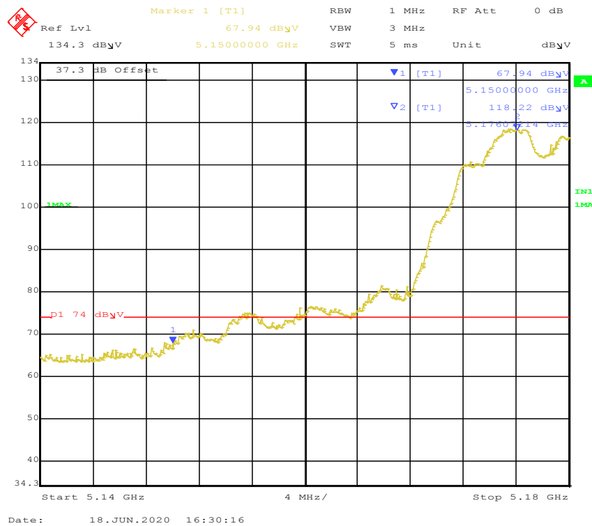
Figure 115: Radiated Emission 5150.0 MHz Edge for 802.11a 5180 MHz – Horz. (Pk)
