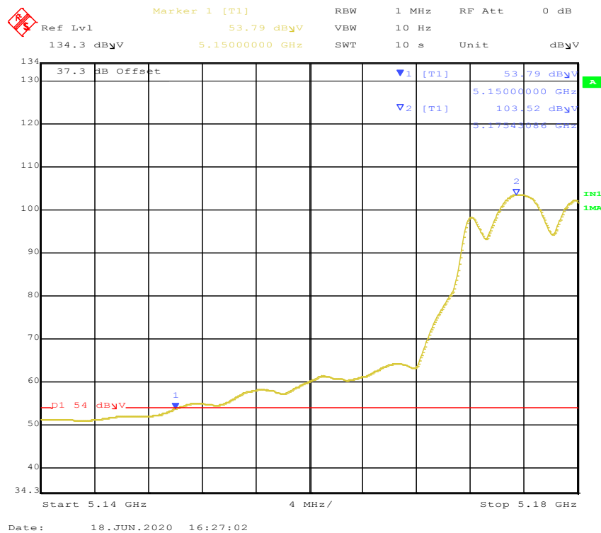
Figure 116: Radiated Emission 5150 MHz Edge for 802.11a 5180 MHz – Horz. (Ave)
