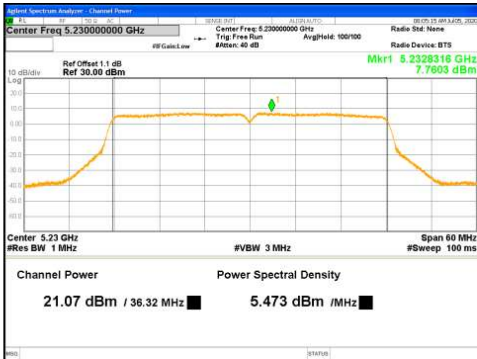
Figure 24: FCC Correlated Max Conducted Power-5230 MHz-802.11n-HT40-MCS0-Ch1
