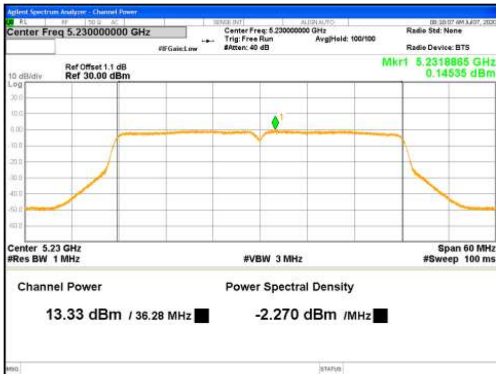
Figure 26: RSS Correlated Max Conducted Power-5230 MHz-802.11n-HT40-MCS0-Ch1
