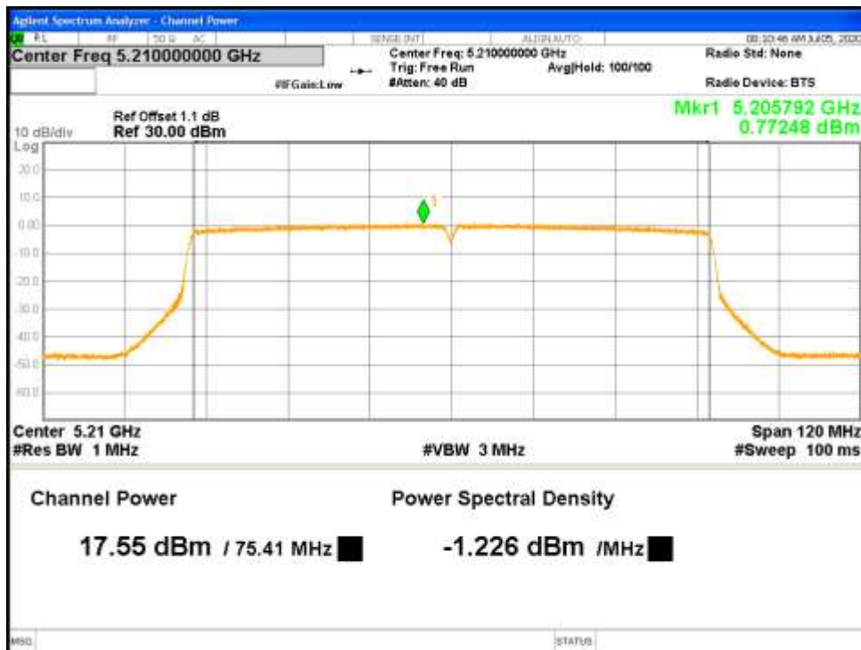
Figure 14: FCC Uncorrelated Max Conducted Power-5210 MHz-802.11ac-VHT80-MCS0-Ch1
