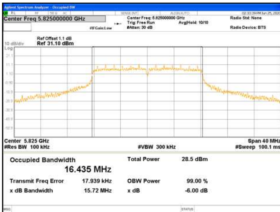
Figure 36: Occupied Bandwidth-5825 MHz-802.11a
