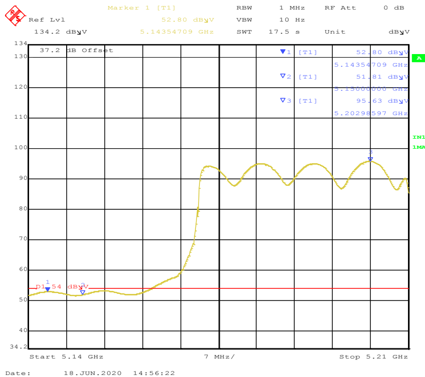
Figure 126: Radiated Emission 5150 MHz Edge for 802.11ac VHT80 5210 MHz – Vert (Ave)
