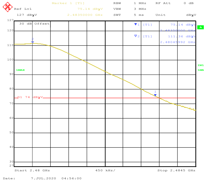
Figure 26: Band-edge-2480 MHz-V-Pk
