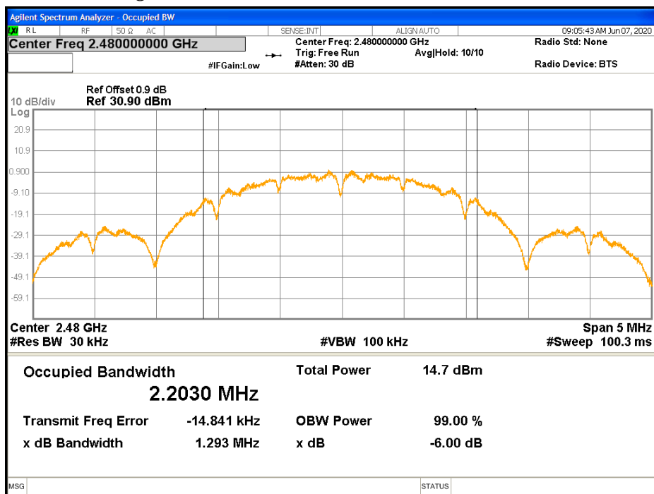
Figure 11: 99% Bandwidth-Transmitter -2480 MHz
