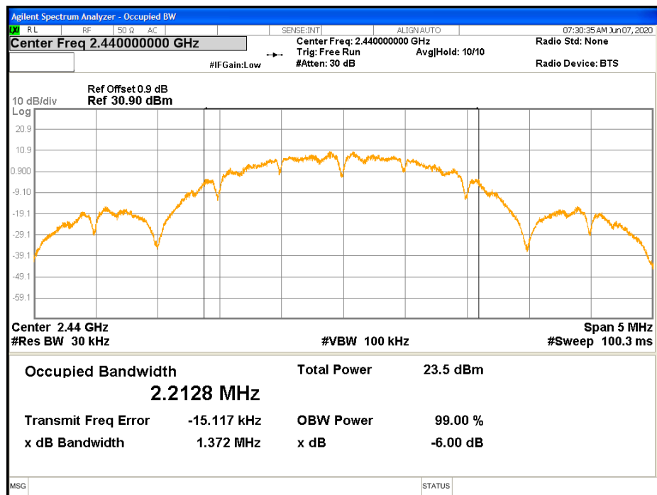
Figure 10: 99% Bandwidth-Transmitter -2440 MHz
