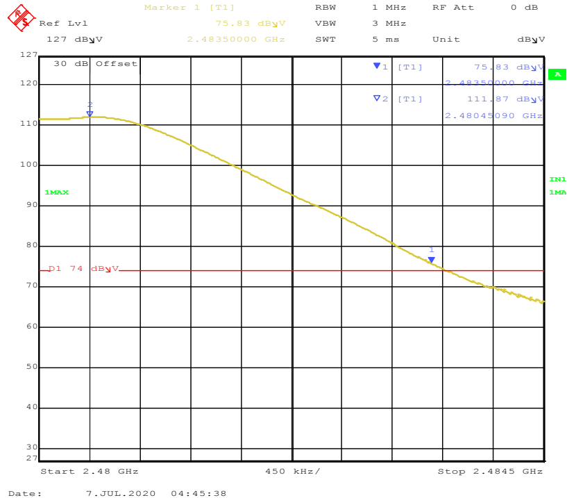
Figure 27: Band-edge-2480 MHz-H-Pk
