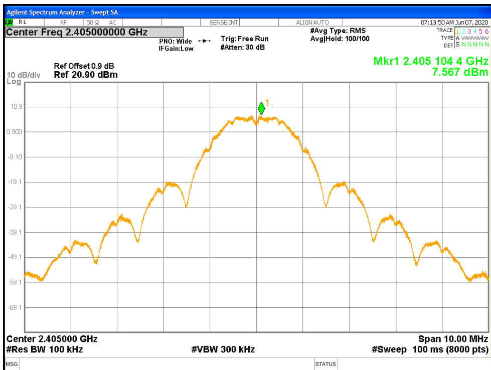
Figure 12: Zigbee Maximum Power Spectral Density-2405 MHz
