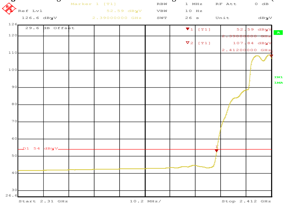
Figure 68: 11g Radiated Emission at the Edge for 2390 MHz – Horz. (Ave)
