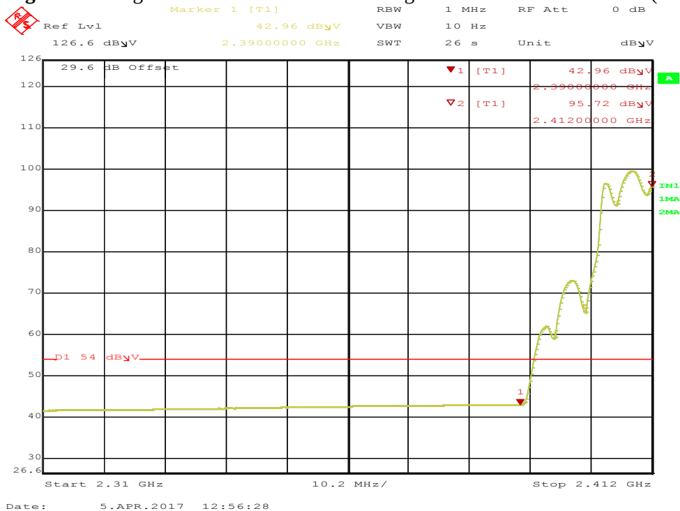
Figure 66: 11g Radiated Emission at the Edge for 2390 MHz – Vert. (Ave)
