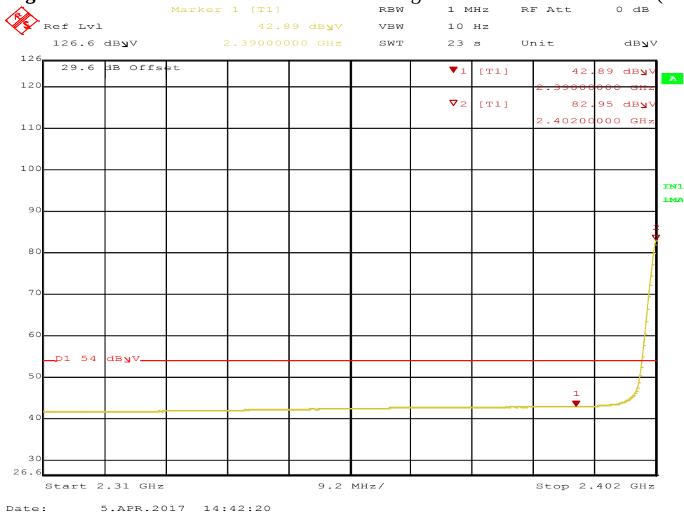
Figure 90: BLE Radiated Emission at the Edge for 2390.0 MHz – Vert. (Ave)
