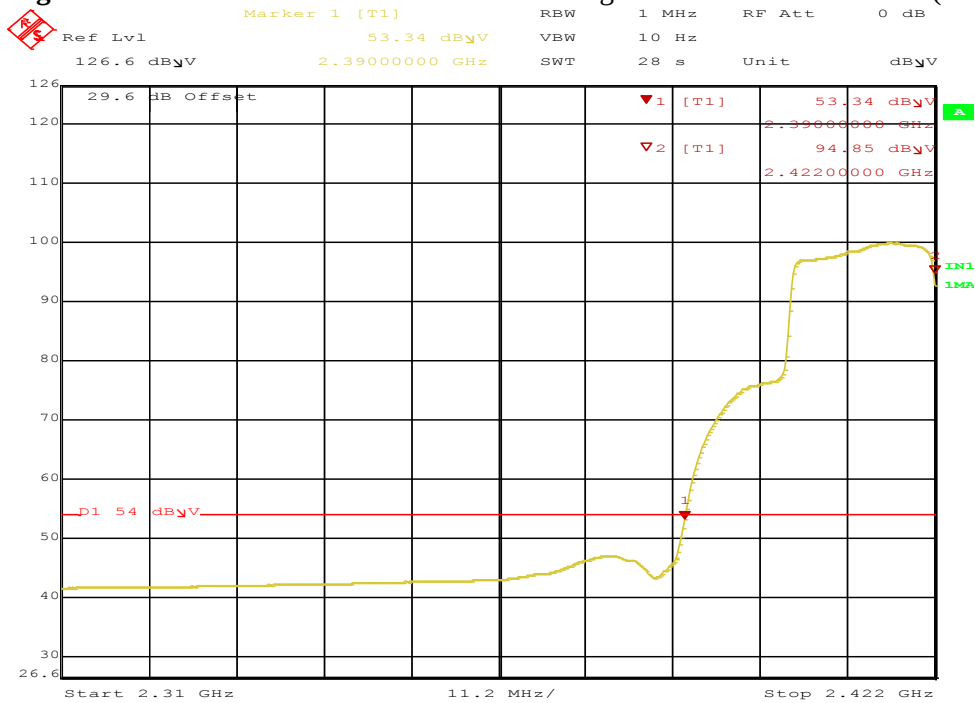
Figure 82: HT40 Radiated Emission at the Edge for 2390 MHz – Horz. (Ave)
