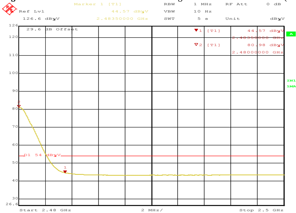
Figure 96: BLE Radiated Emission at the Edge for 2483.5 MHz – Vert. (Ave)
