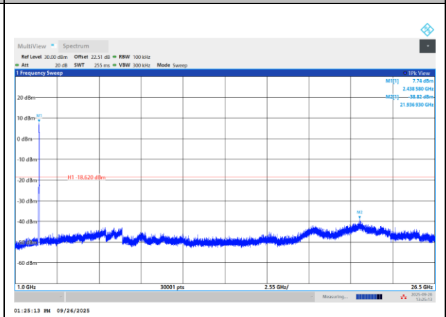
Spurious Emission 1GHz~26.5GHz
