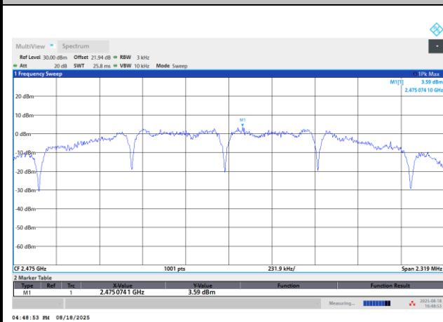
Power Density (dBm/3kHz) Plot Channel 25
