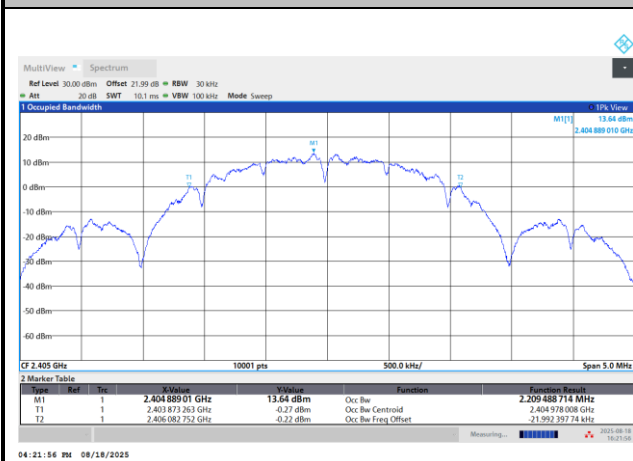
99% Occupied Bandwidth Plot on Channel 11
