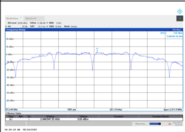
Power Density (dBm/3kHz) Plot Channel 18
