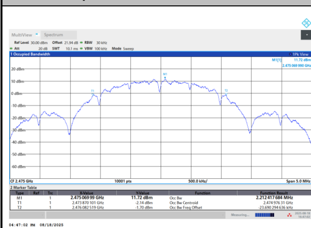
99% Occupied Bandwidth Plot on Channel 25
