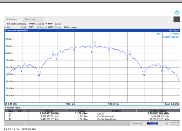
99% Occupied Bandwidth Plot on Channel 18
