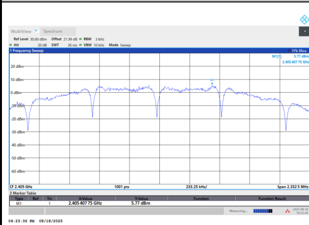
Power Density (dBm/3kHz) Plot Channel 11
