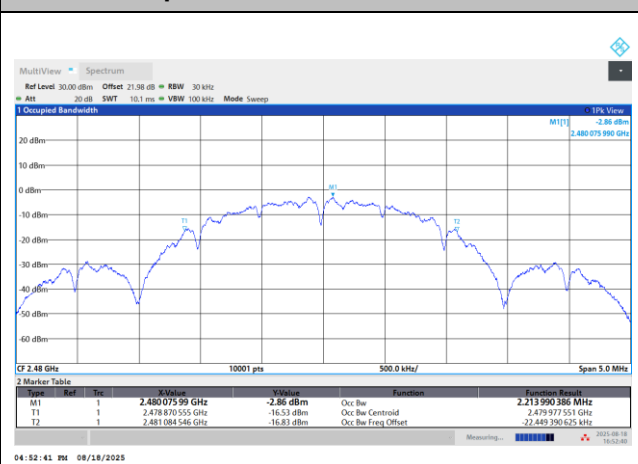
99% Occupied Bandwidth Plot on Channel 26
