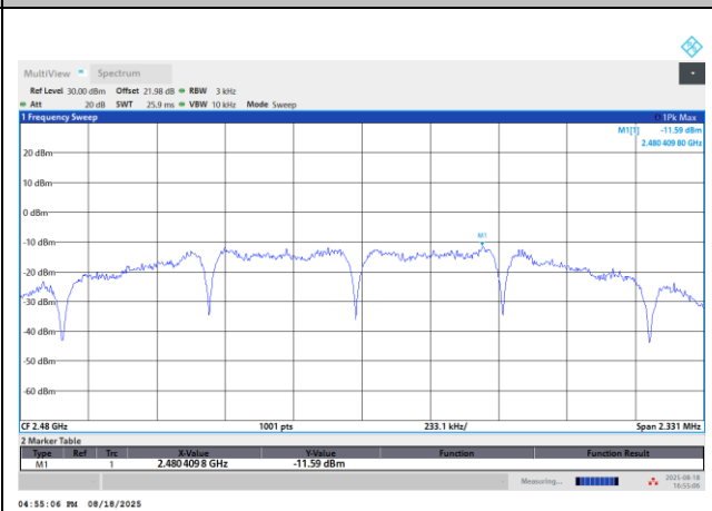
Power Density (dBm/3kHz) Plot Channel 26
