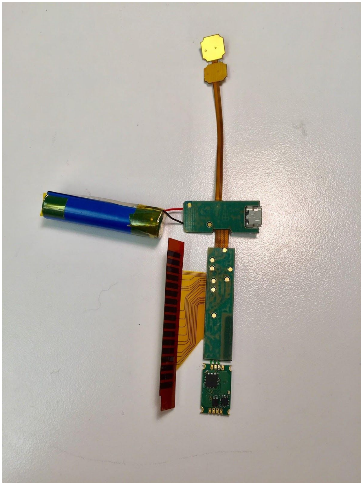
Figure 6: Printed Clrcuit Board View From Bottom
