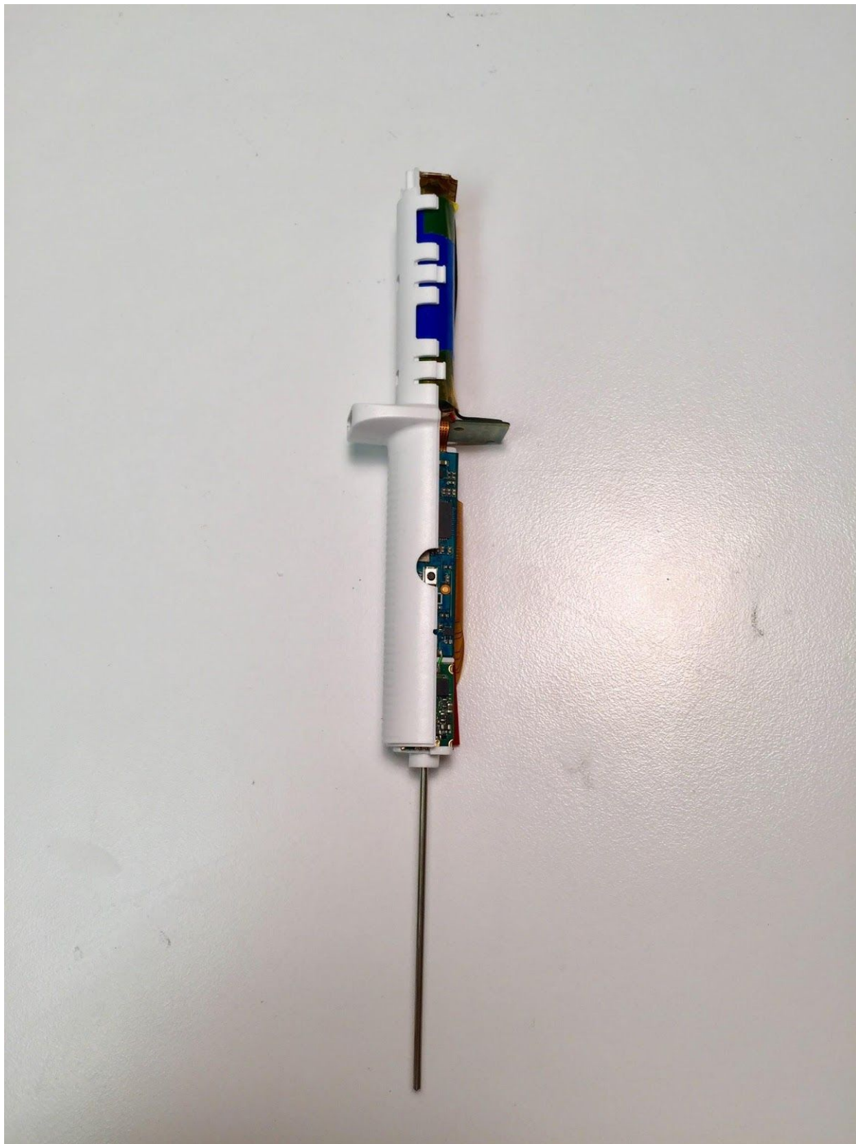
Figure 3: Needle Opened to Expose Printed Circuit Board
