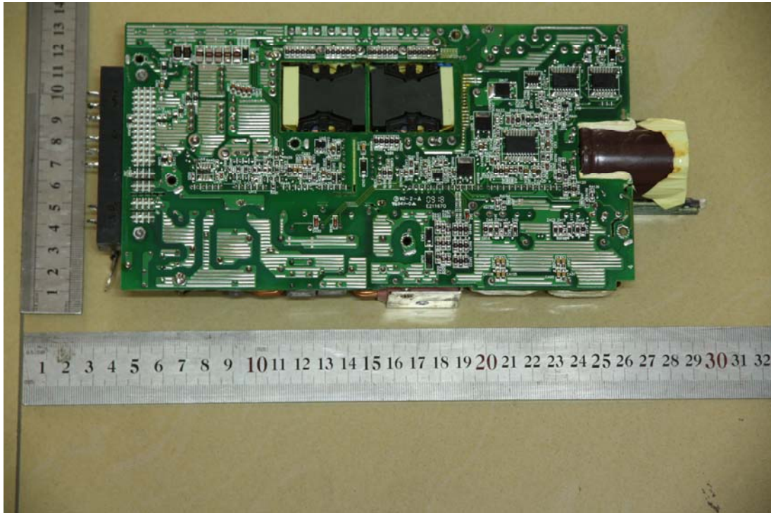
Power supply mainboard Bottom View
