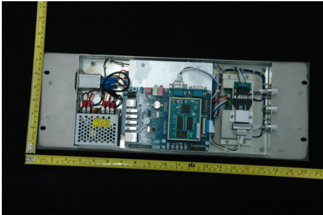
Uncover View
