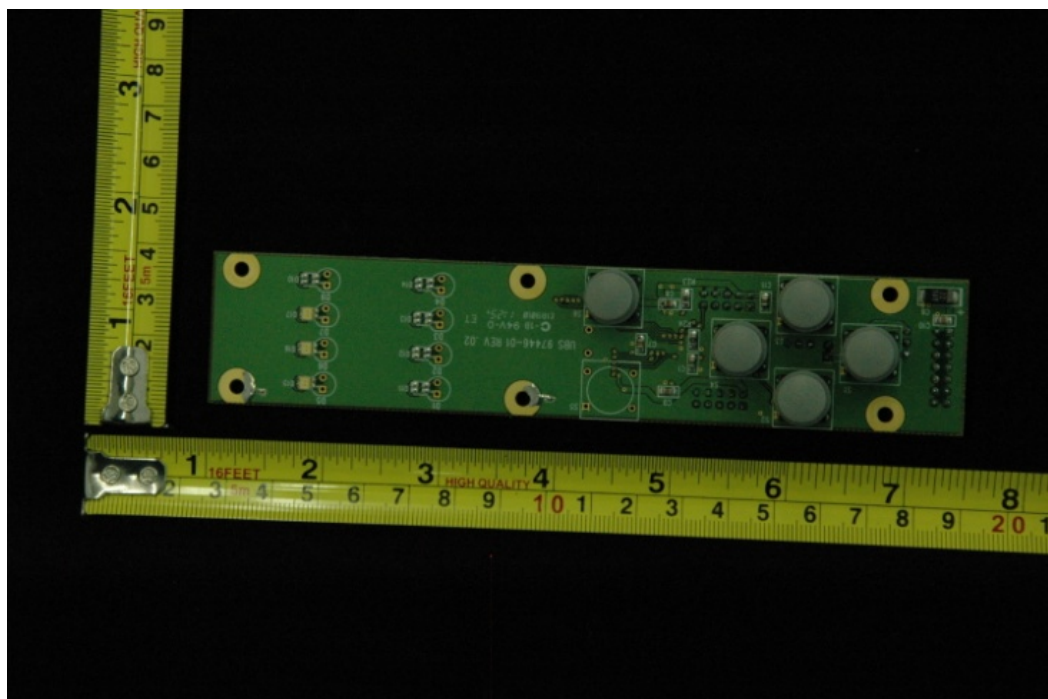
Key board Top View
