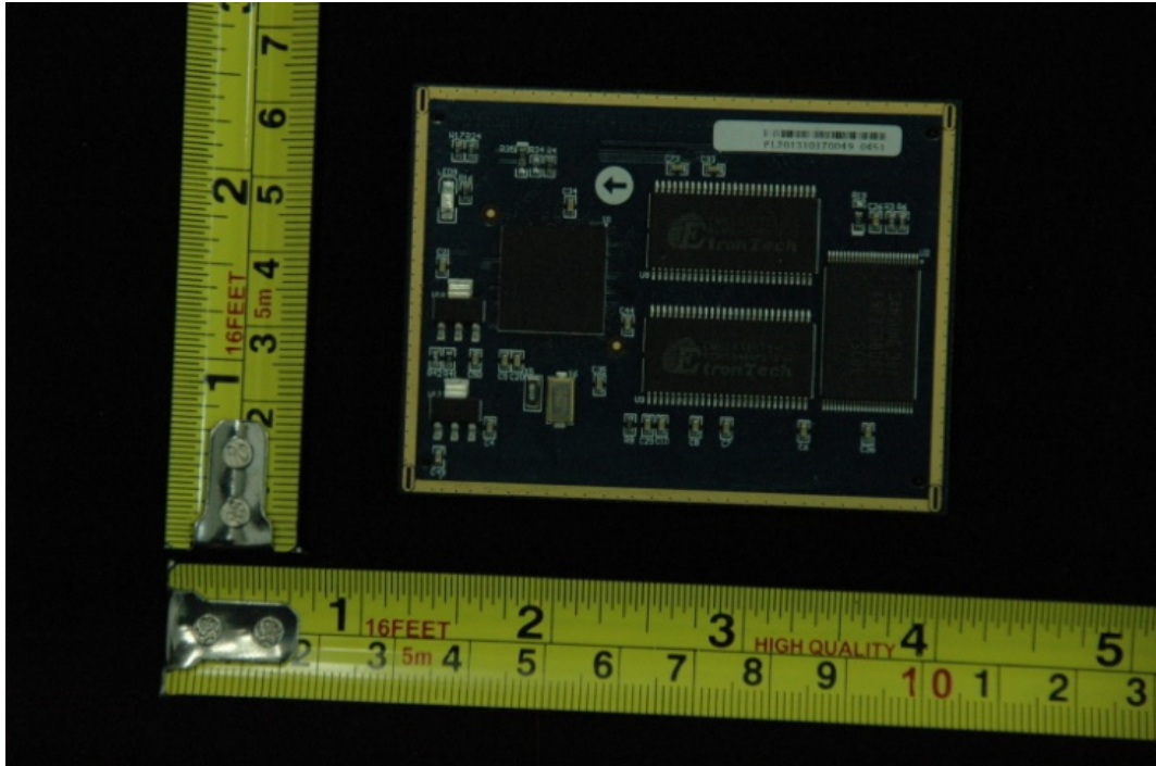
Core board Top View
