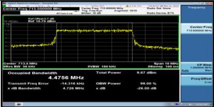
(Channel Bandwidth: 5 MHz)_HCH_QPSK_25RB#0
