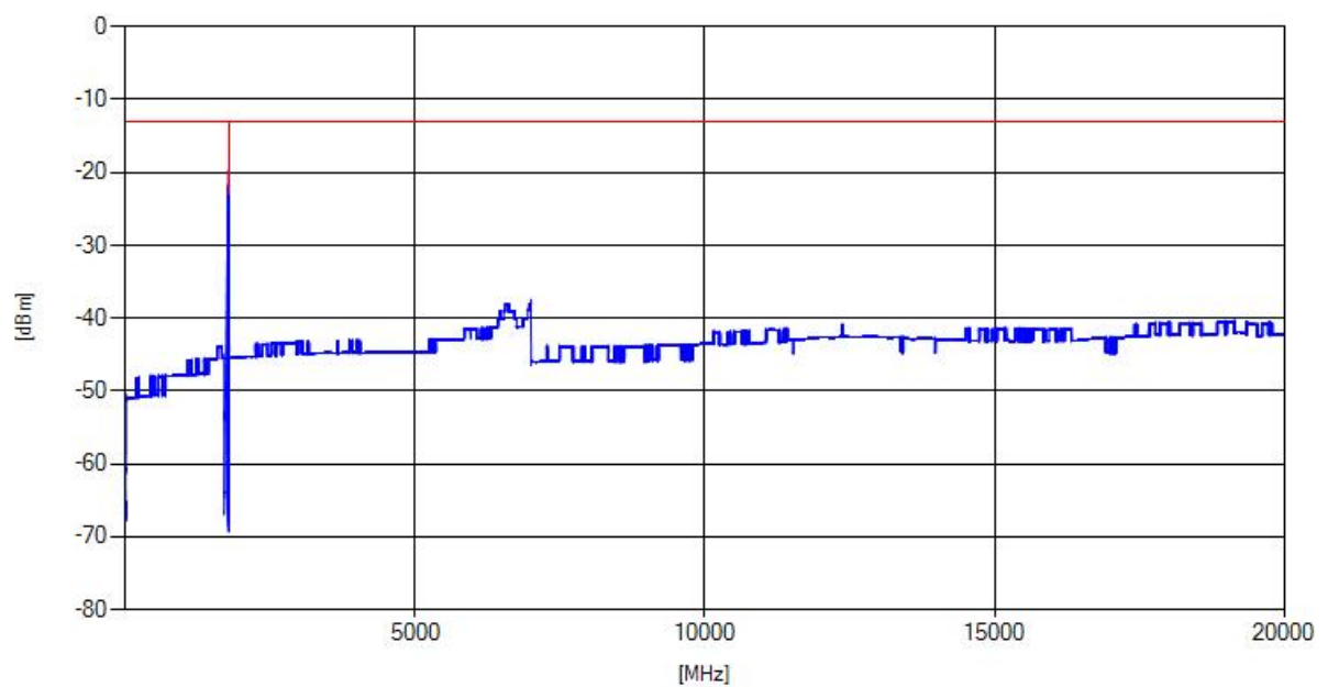
NB-IoT eFDD66 QPSK, Channel = high
