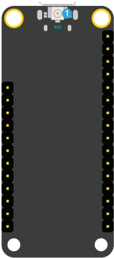
1 u.FL CONNECTOR FOR NFC ANTENNA
