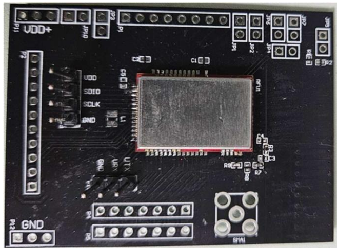
Figure 1: Gwell GW-LLCC68 DK with PCB Antenna
