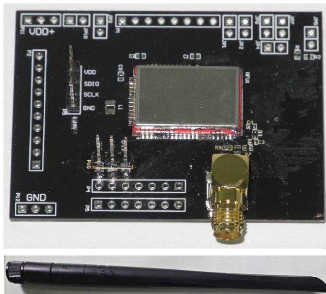
Figure 2: Gwell GW-LLCC68 DK with SMA Antenna
