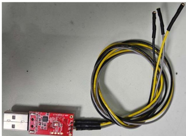
Figure 3: Gwell Wiring USB connector with UART signal
