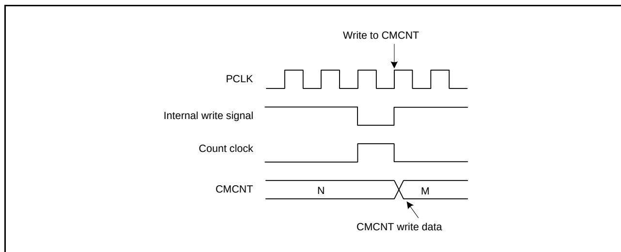
Figure 27.6 Conflict between CMCNT Counter Writing and Incrementing
