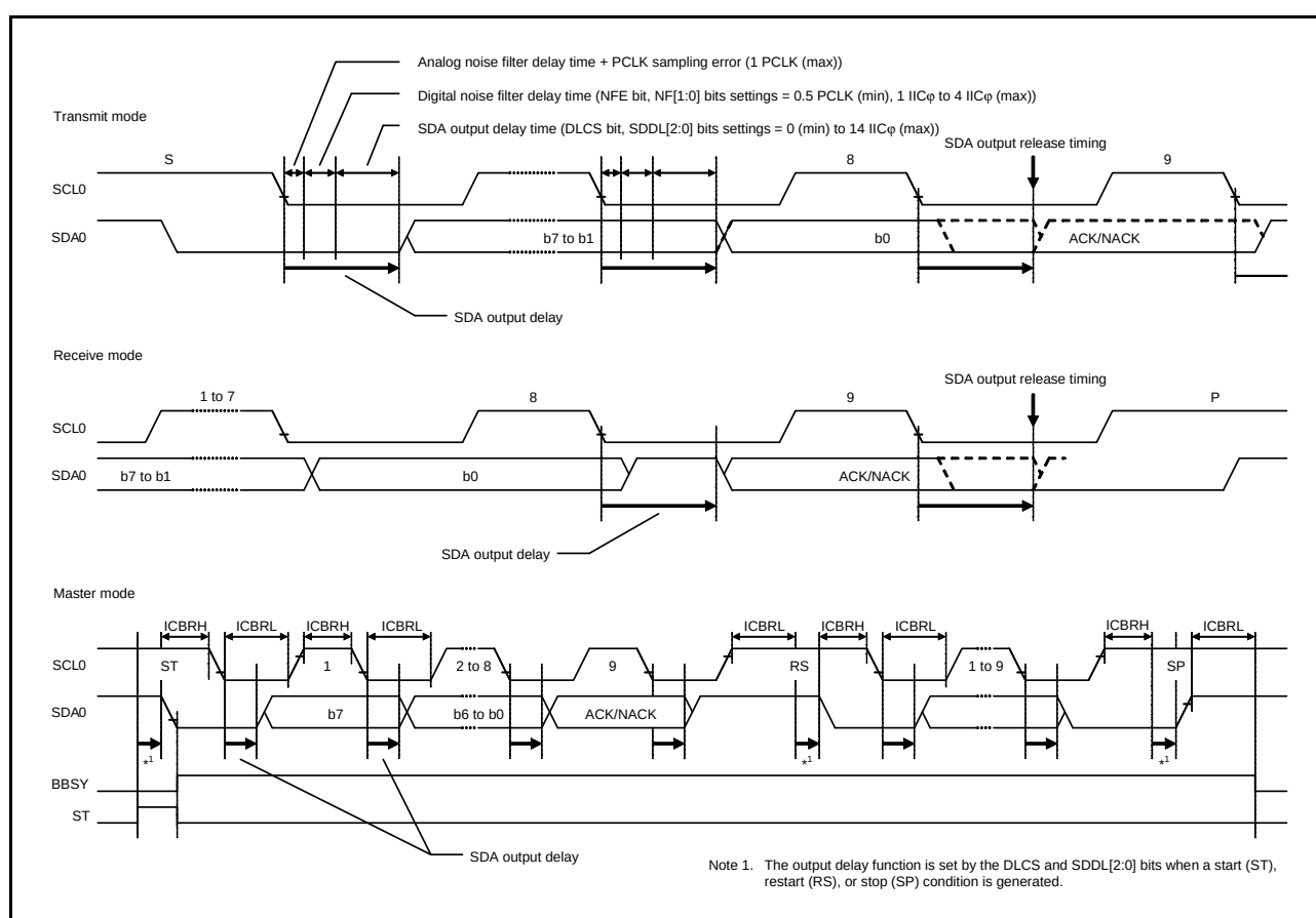
Figure 35.22 SDA Output Delay Function
