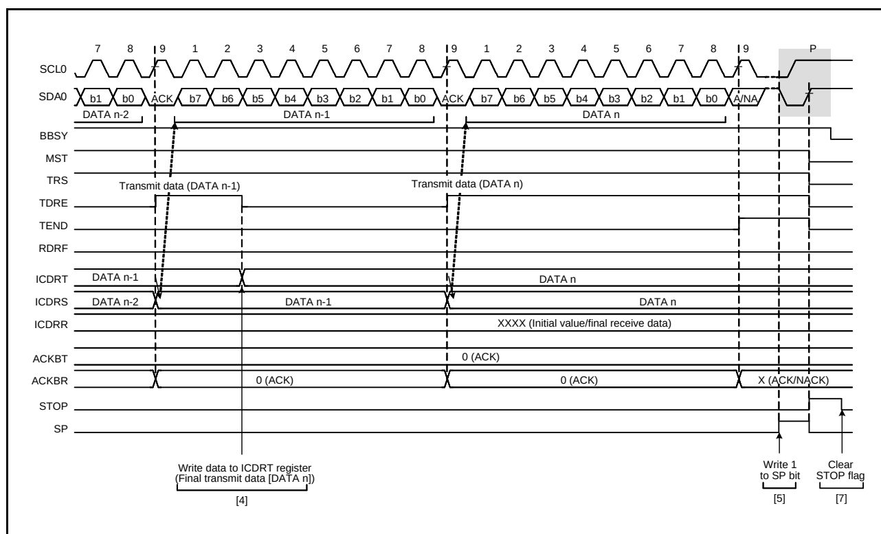
Figure 35.9 Master Transmit Operation Timing (3)
