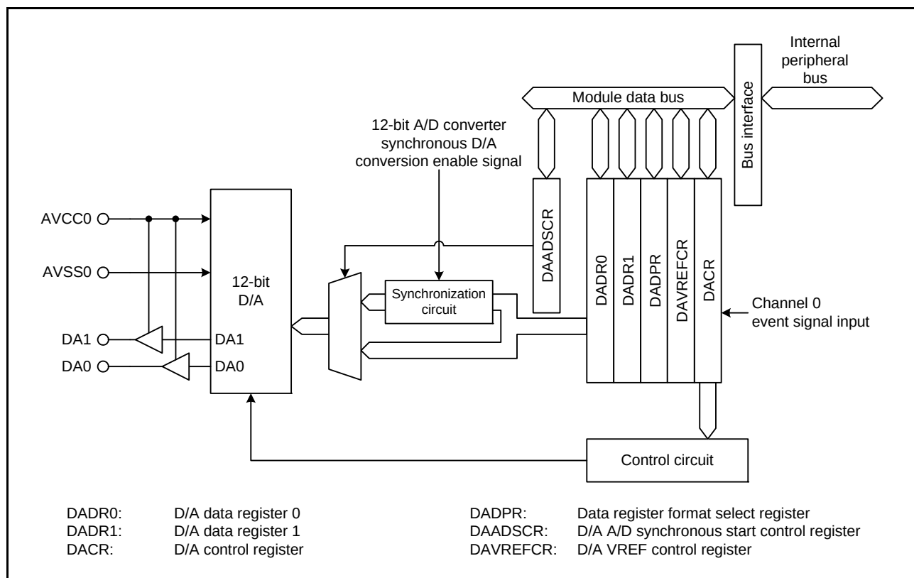
Figure 45.1 Block Diagram of 12-Bit D/A Converter
