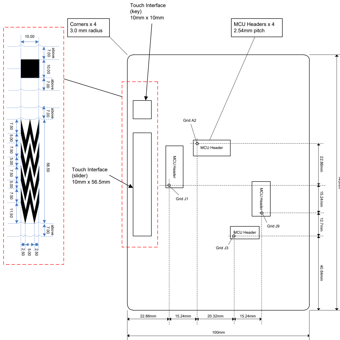
Figure 3-2: Board Dimensions
